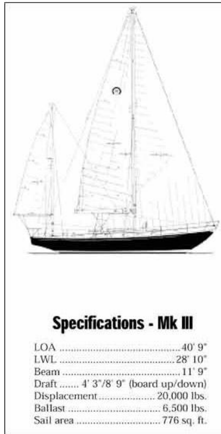
Hinckley Bermuda 40
